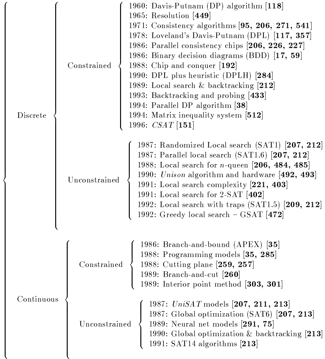
FIGURE 5. Some typical algorithms for the SAT problem.
